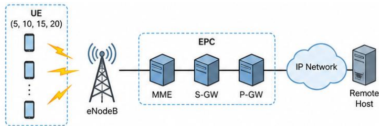
Figure 2. 4G LTE Network Topology
